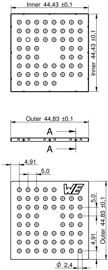
sectional drawing A-A
