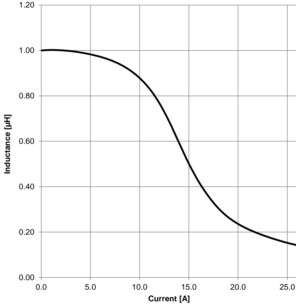
Typical Inductance vs. Current Characteristics - Three Turns:
