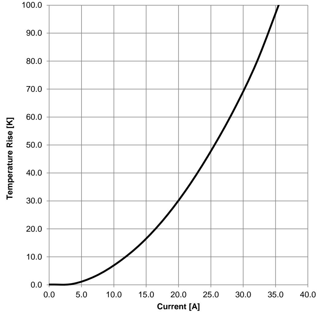
Typical Temperature Rise vs. Current Characteristics - Three Turns:
