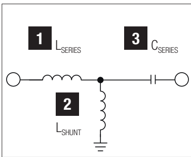
T matching for Point A
