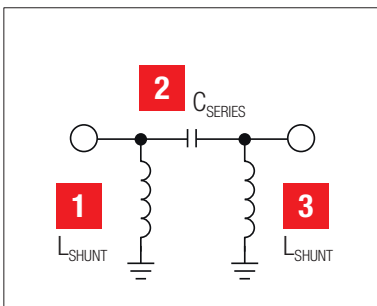
Pi matching for Point B
